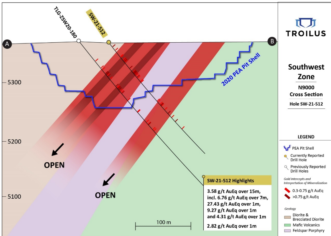
Figure 2: Section N9000; View of drill hole SW-21-512
